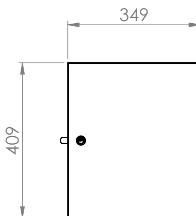
DETAIL E
