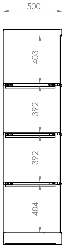
SECTION B-B
