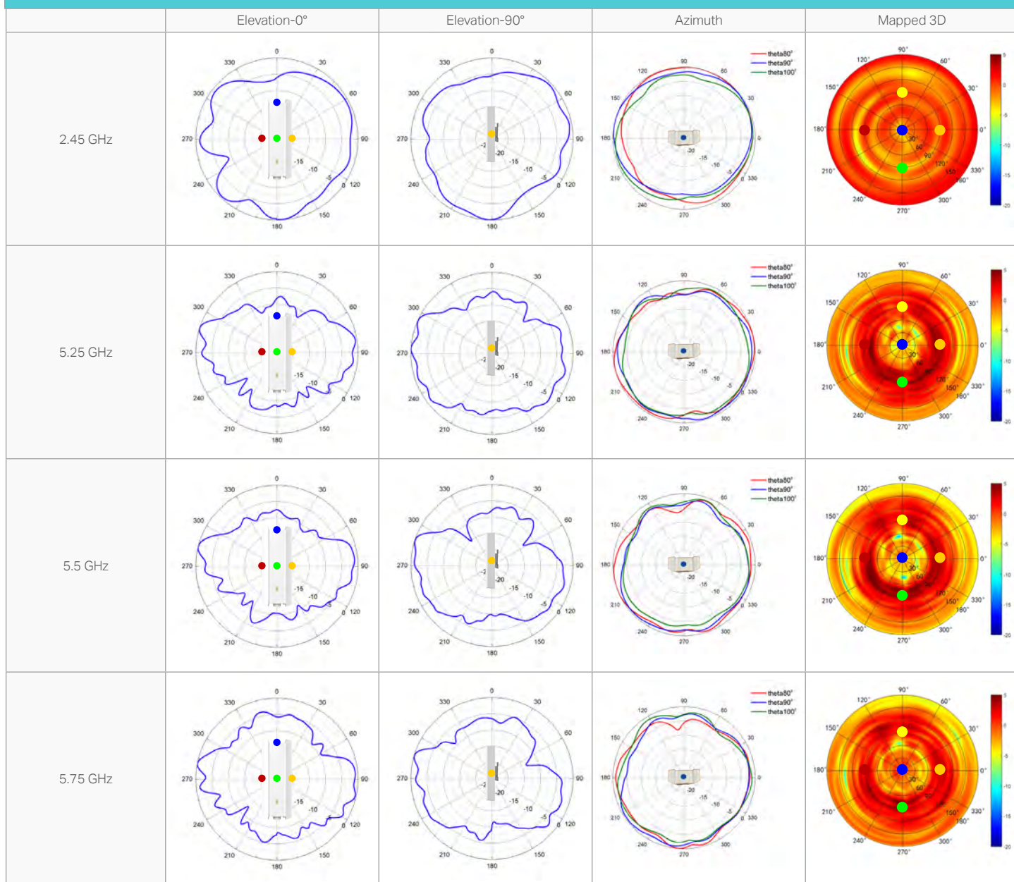
EAP610-Outdoor
