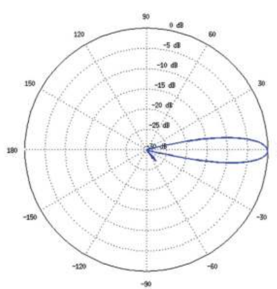
Vertical Elevation
