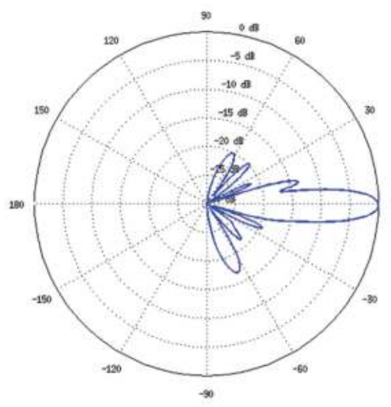
Horizontal Elevation
