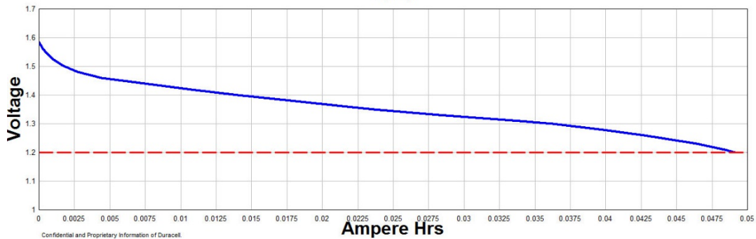
15K Ohm Cont. to 1.2V Capacity
