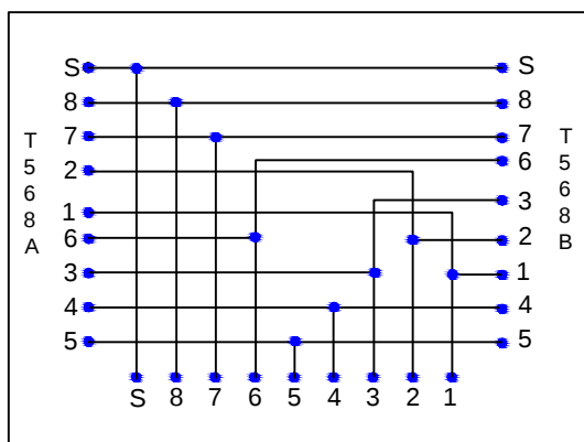
Pin-Belegung / Pin assignment
