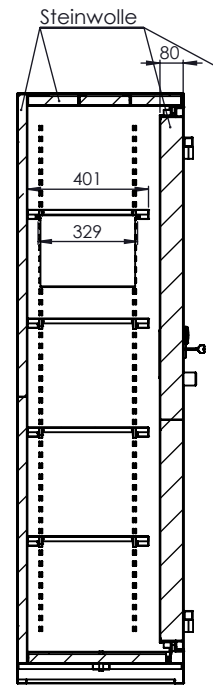
SECTION B-B
