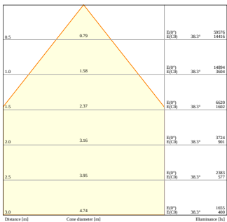
HB DA P 150W 840 110DEG IP66 WITH REFLECTOR
