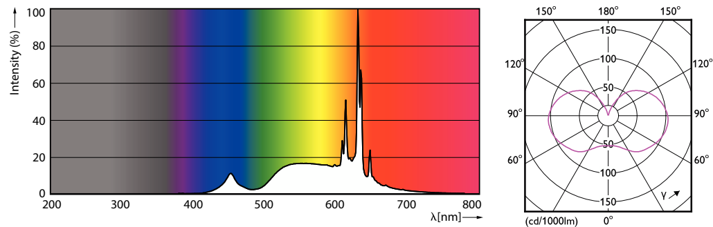
Spectral Power Distribution Colour
