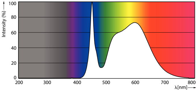
Spectral Power Distribution Colour - MAS LEDtube 1200mm UO 13.5W 840 T8 EELB
