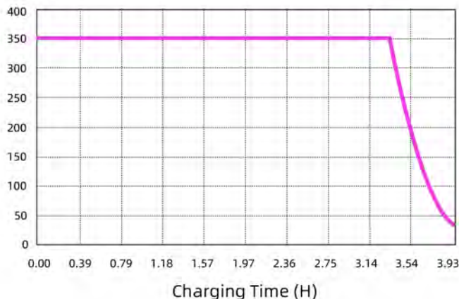
Charging Current Diagram By USB-C (Input Power 5V 0.5A)
