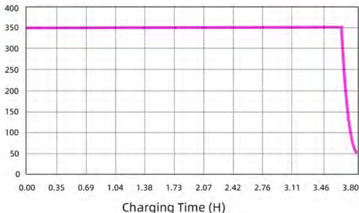
Charging Current Diagram By XTAR L8 charger
