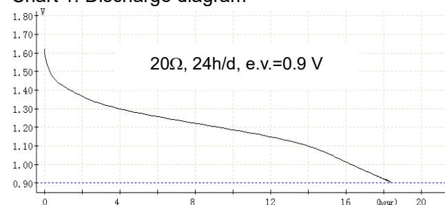
Chart 1. Discharge diagram
