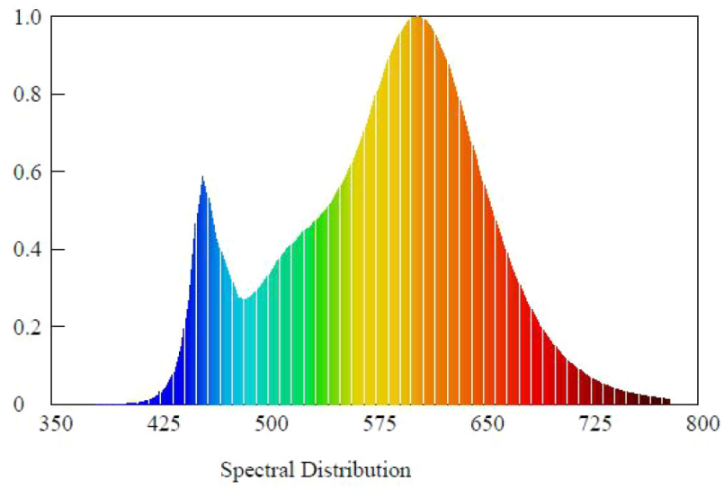
Spectral power distribution (3000K)
