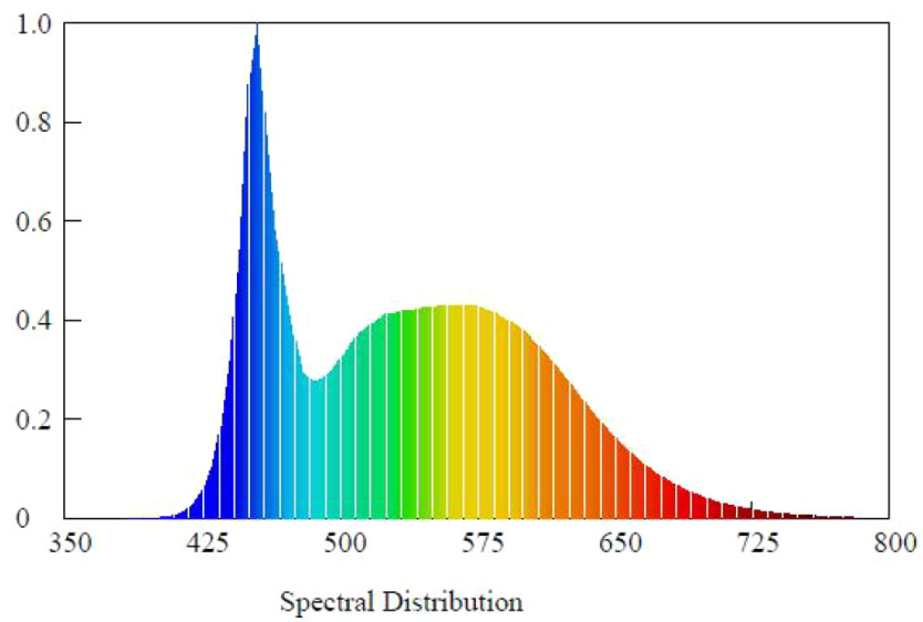
Spectral power distribution (6500K)
