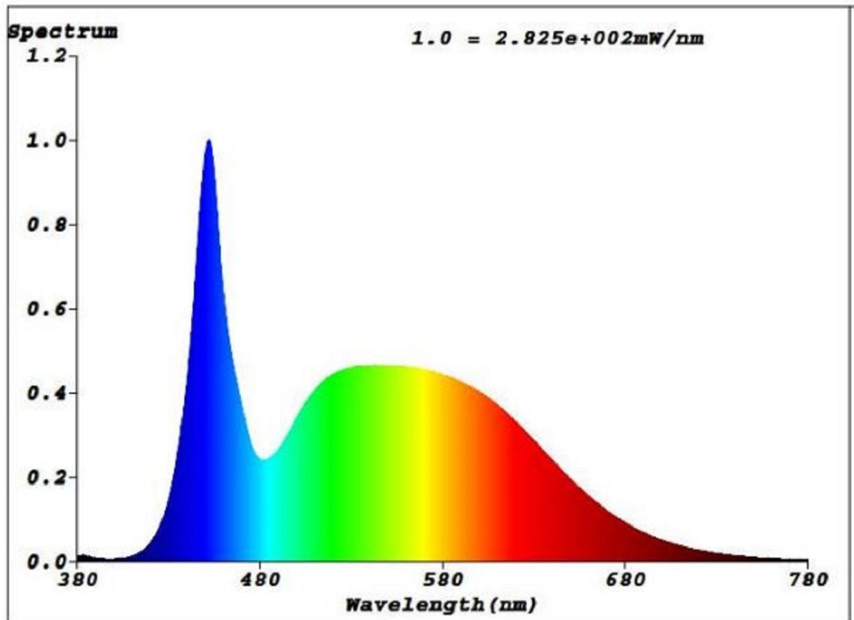
Photo 1: Spectrum of 6500K
