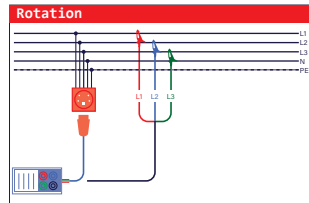
Fig. 32: Connection diagram for phase sequence
