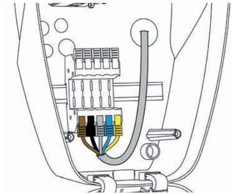
Fig. 8: Power supply connection (example)
