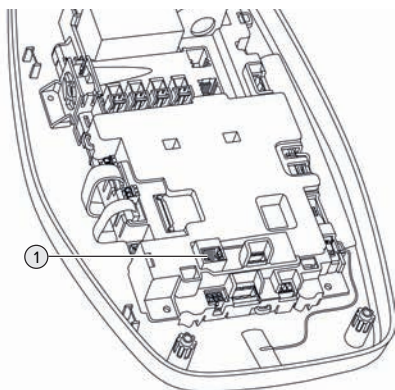
Fig. 12: Porta Ethernet
