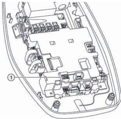
Fig. 12: Ethernet port
