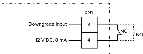
Fig. 15: Schematic circuit diagram: Connection of an external switching contact (default setting: NO)
