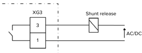
Fig. 10: Schematic circuit diagram: Connecting an external shunt release
