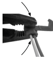
Figure 5: Pressing in the small contact plates
