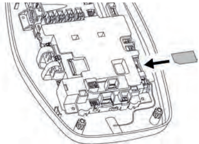
Fig. 11: Inserting the SIM card
