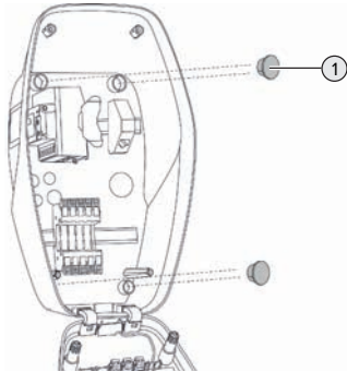
Fig. 7: Sealing plugs
