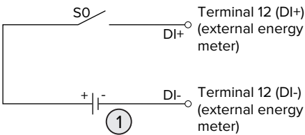
Fig. 17: Control via a coupling relay and additional power supply (when in delivery state)
