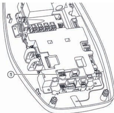
Fig. 13: Ethernet port
