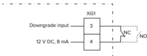
Fig. 12: Schematic circuit diagram: Connection of an external switching contact (default setting: NC)
