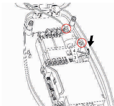
Fig. 11: Downgrade input connection
