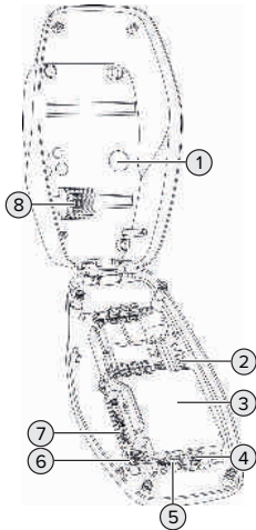
Fig. 3: Interior view
