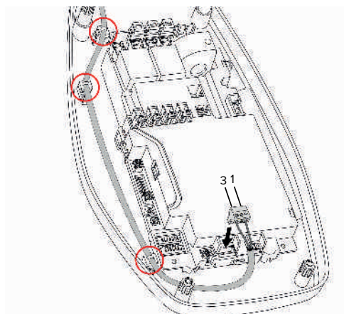
Fig. 7: Shunt release connection
