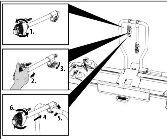
Figure 9: Assembly of frame holder
