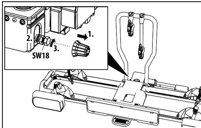
Figure 15: Adjustment of the quick lock
