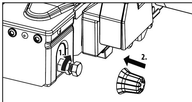
Figure 16: Adjustment of the quick lock
